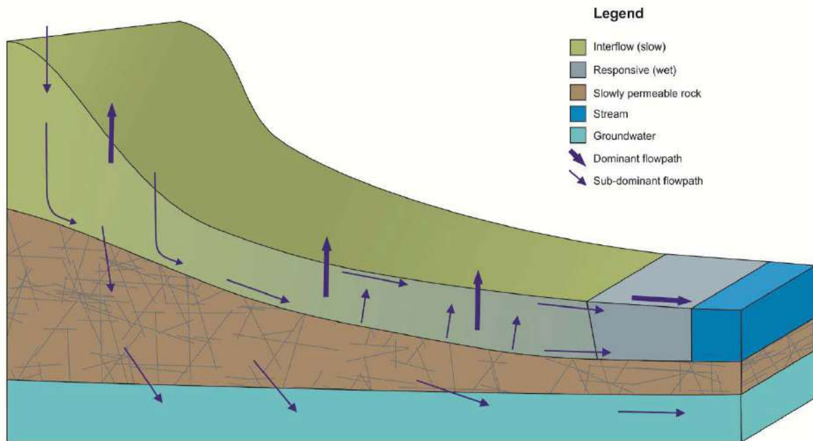
Figure 6.12. Conceptual hydrological response of a Class 11 hillslope.
