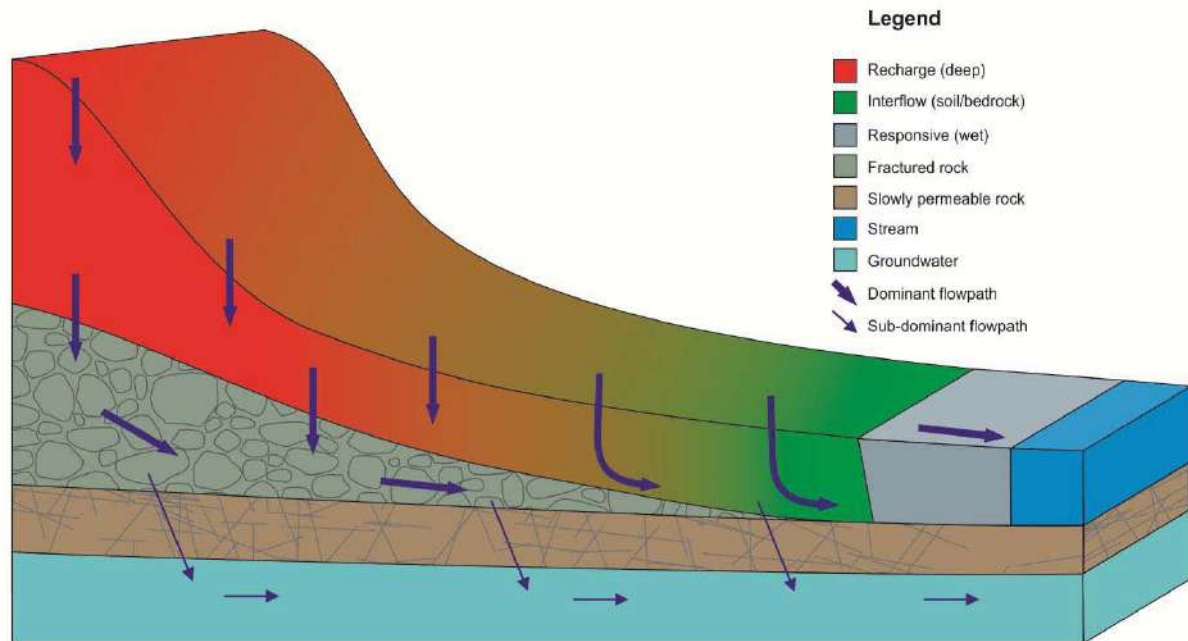
Figure 6.11. Conceptual hydrological response of a Class 10 hillslope.
