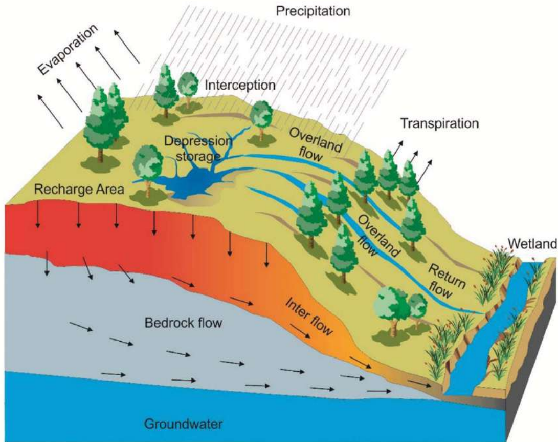
Figure 2.2. Hydrological flowpaths at hillslope scale.
