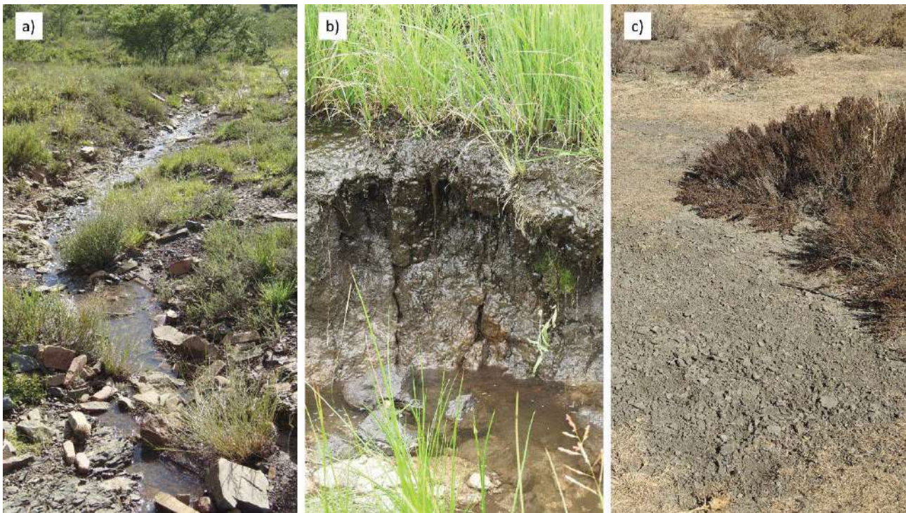
Figure 5.3. Examples of responsive soil: a) Responsive (shallow) – overland flow is generated due to low storage capacity, b) Responsive (wet) – overland flow is generated by saturation excess and c) Responsive (Hortonian) – overland flow will be generated due to crusting and low infiltration rates.
