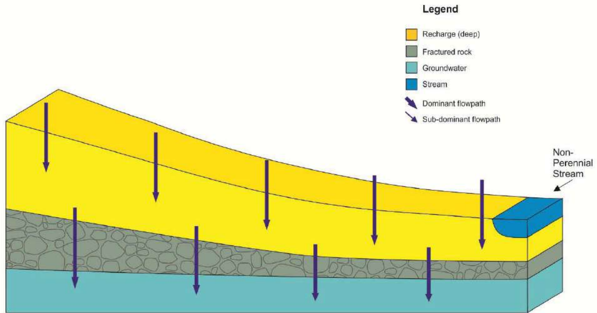
Figure 6.9. Conceptual hydrological response of a Class 8 hillslope.
