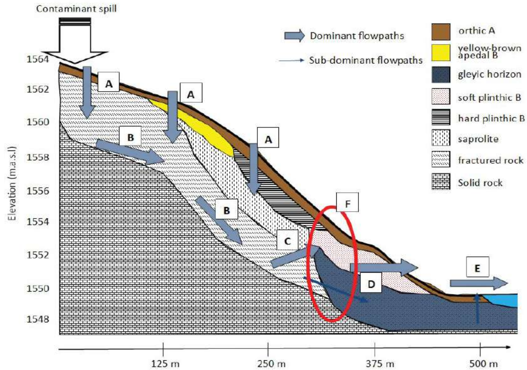
Figure 11.7. Conceptual hydrological flowpaths derived from a transect soil survey to determine the migration routes of pollutants.
