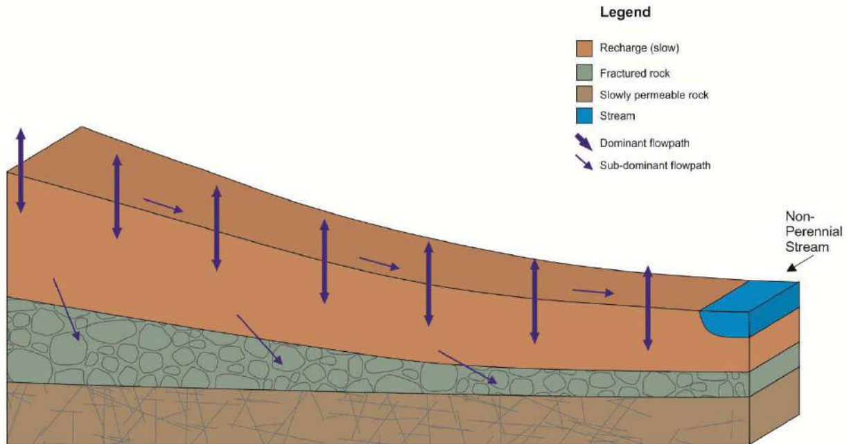
Figure 6.8. Conceptual hydrological response of a Class 7 hillslope.
