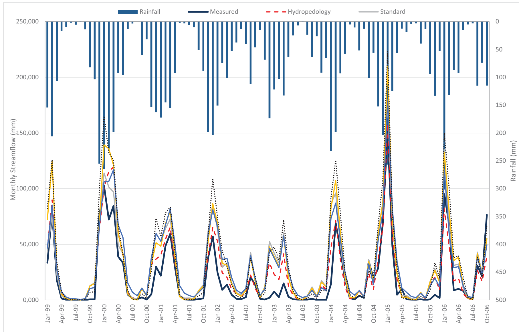
Figure 12.2. Monthly measured and simulated streamflow for the Weatherley catchment using different soil inputs.
