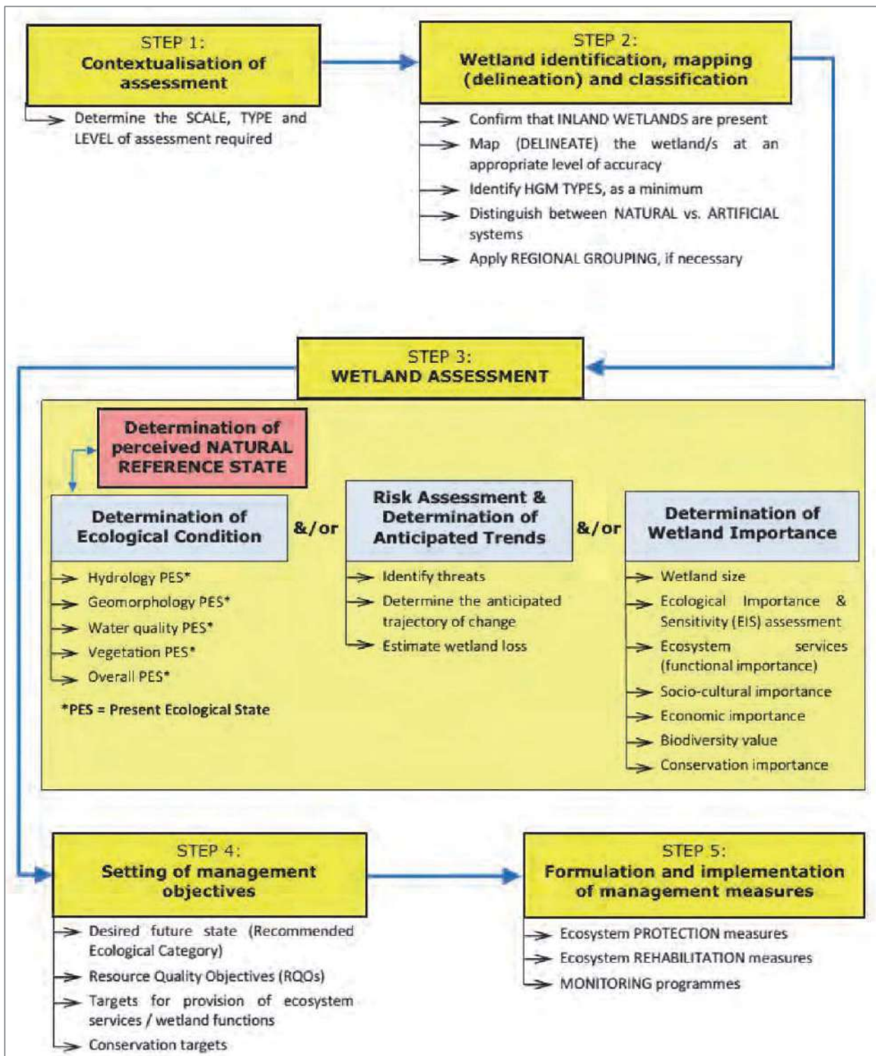
Figure 7.1. Decision-support framework for wetland assessment in South Africa (Ollis et al., 2014).
