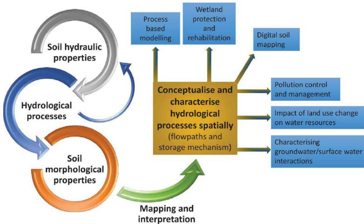
Figure 1.1. The basis of hydropedology and its implication (Van Tol et al., 2017).
