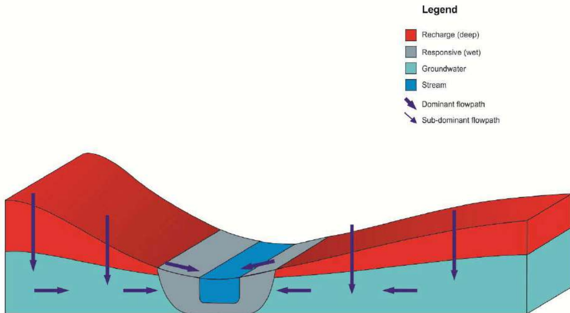
Figure 6.3. Conceptual hydrological response of a Class 2 hillslope.
