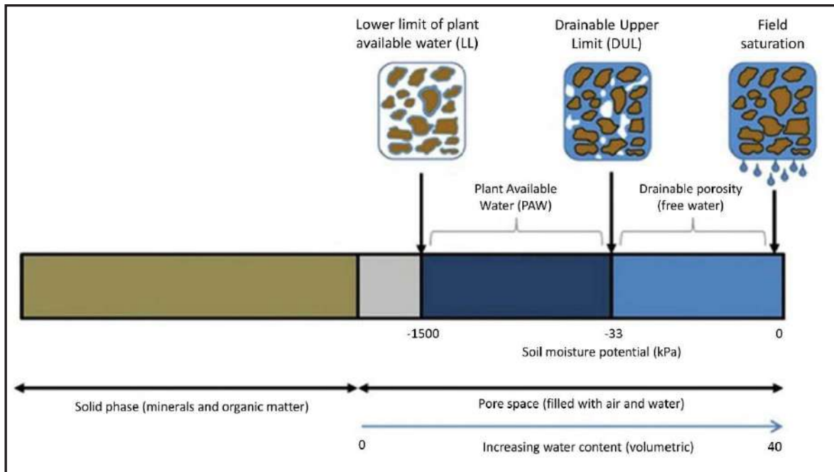
Figure 3.6. Soil as a three-phase system with different soil water retention characteristics: Lower limit (LL) of plant available water (PAW), Drained Upper Limit (DUL) and saturation (altered from O'Geen, 2013).
