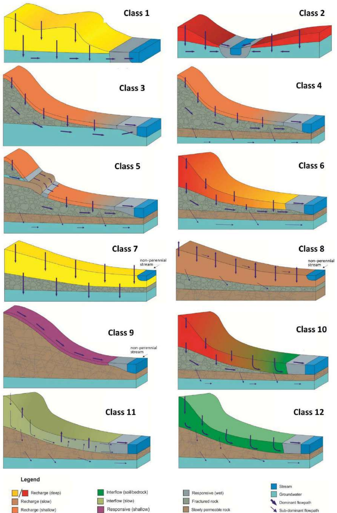
Figure A. Graphical summary of hillslope hydropedological response classes.
