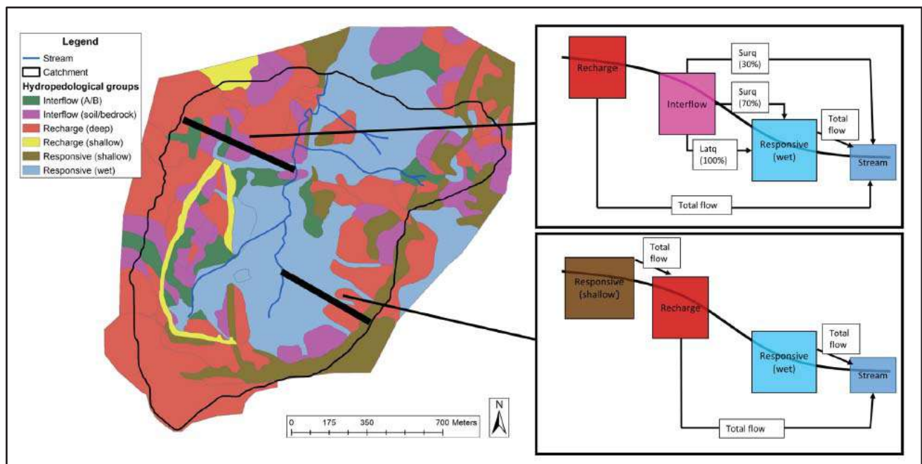
Figure 12.1. Distribution of hydropedological soil groups in the Weatherley catchment with typical routing in two hillslopes (Van Tol et al., 2021b). Latq = Lateral flow; Surq = Surface runoff.
