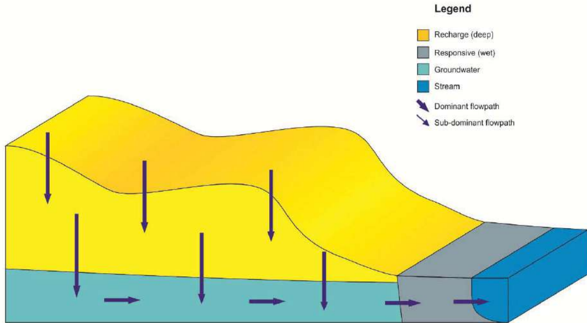
Figure 6.2. Conceptual hydrological response of a Class 1 hillslope.
