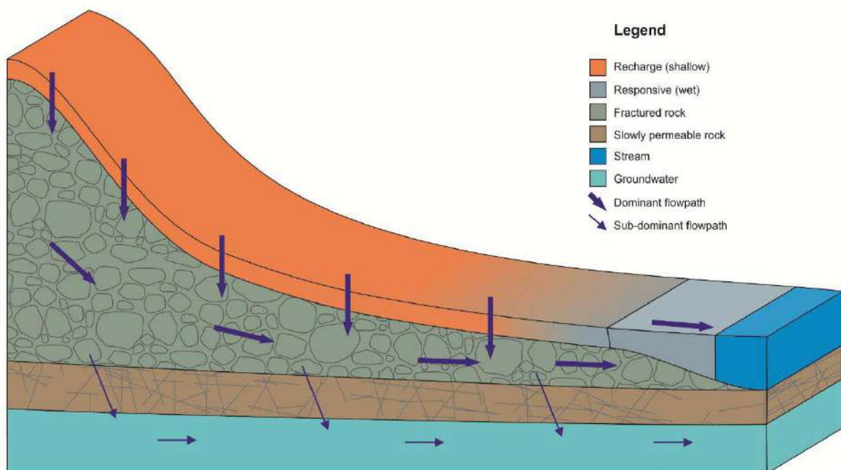
Figure 6.5. Conceptual hydrological response of a Class 4 hillslope.
