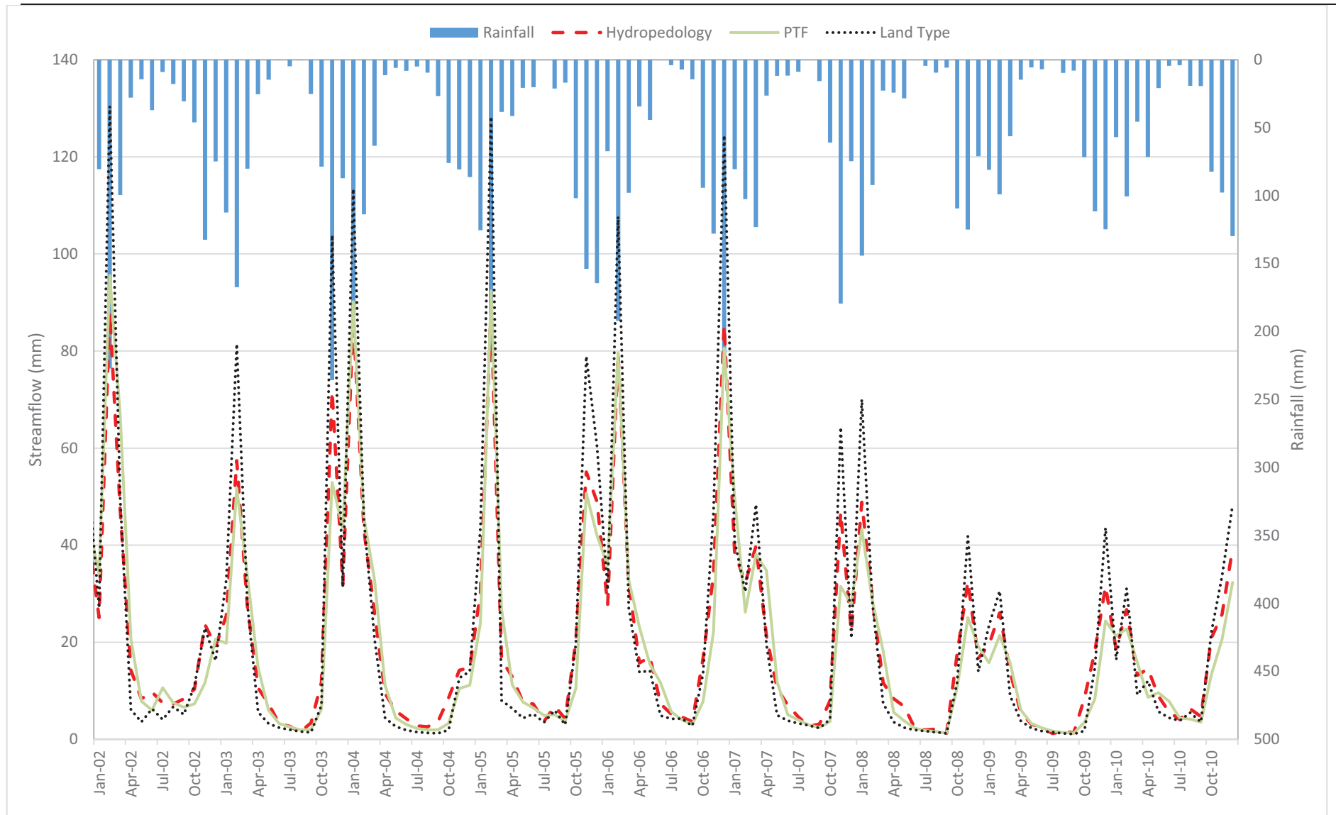
Figure 12.5. Monthly simulated streamflow for the Mpumalanga Highveld catchment using different soil inputs.
