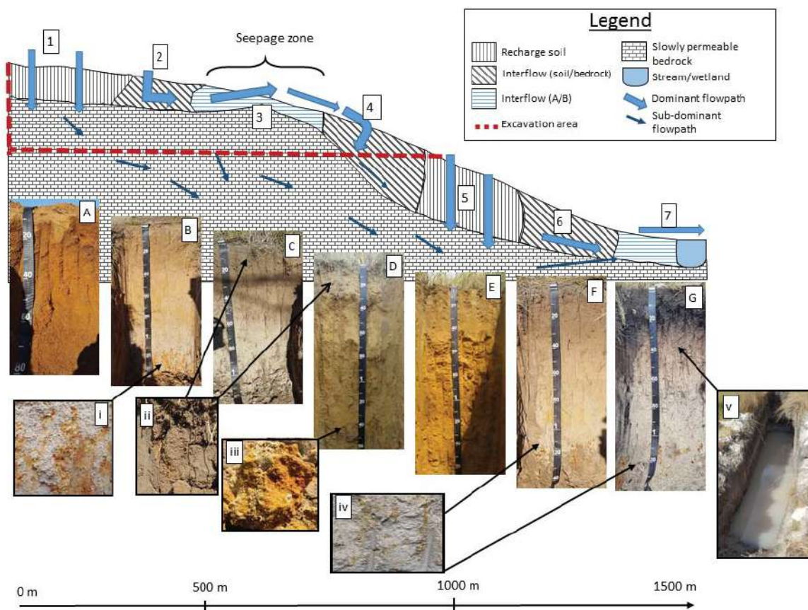
Figure 11.1. Pedosequence of representative soil profiles and their hydrolopedological behaviour of a hillslope in the Eastern Highveld of South Africa.
