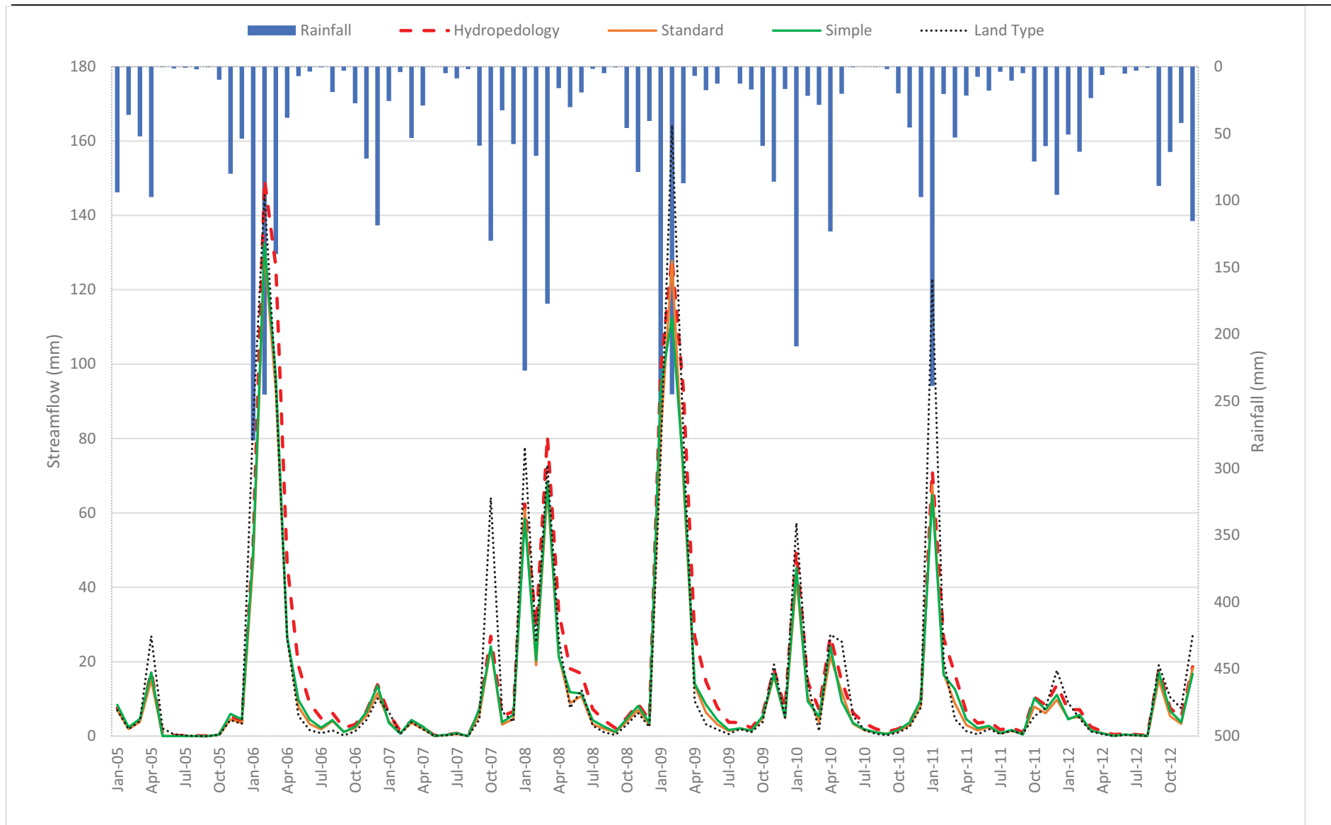
Figure 12.3. Monthly simulated streamflow for the Cosmo City catchment using different soil inputs.
