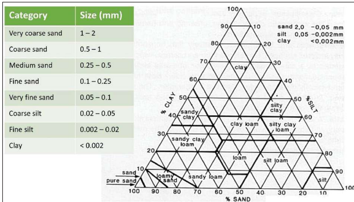
Figure 3.4. Particle size categories and texture triangle to describe textural classes.
