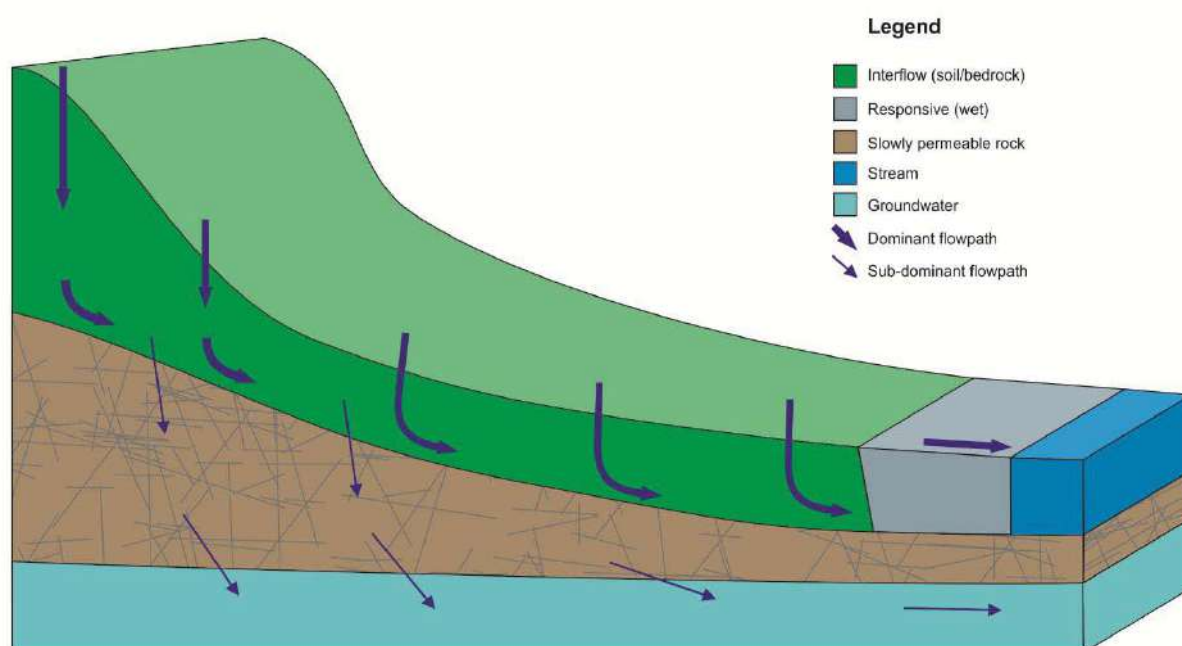
Figure 6.13. Conceptual hydrological response of a Class 12 hillslope.
