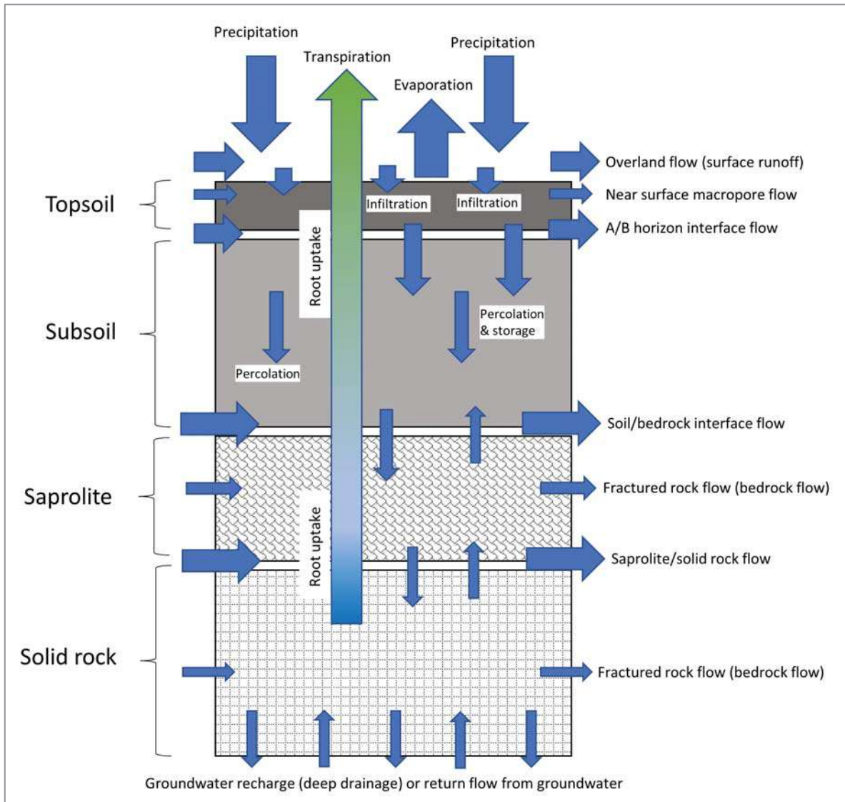
Figure 2.1. Vadose zone water balance.
