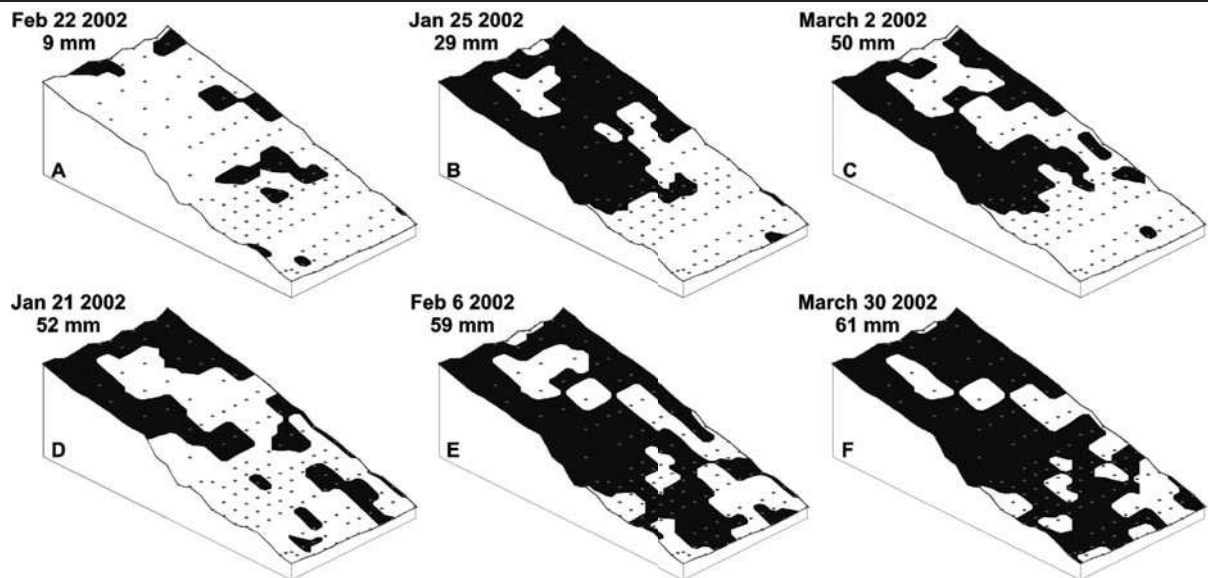
Figure 2.4. Subsurface saturation in the Ponola hillslope with varying rainfall amounts (Tromp-Van Meerveld and McDonnell, 2006b).
