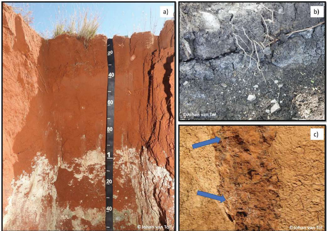
Figure 3.2. \text{CaCO}_3 accumulations a) below red apedal horizon in a Kimberley soil form near Hope Town, b) between structural units in a Vertic horizon near Rustenburg, and c) in infilled root channels of an Augrabies soils near Bedford.
