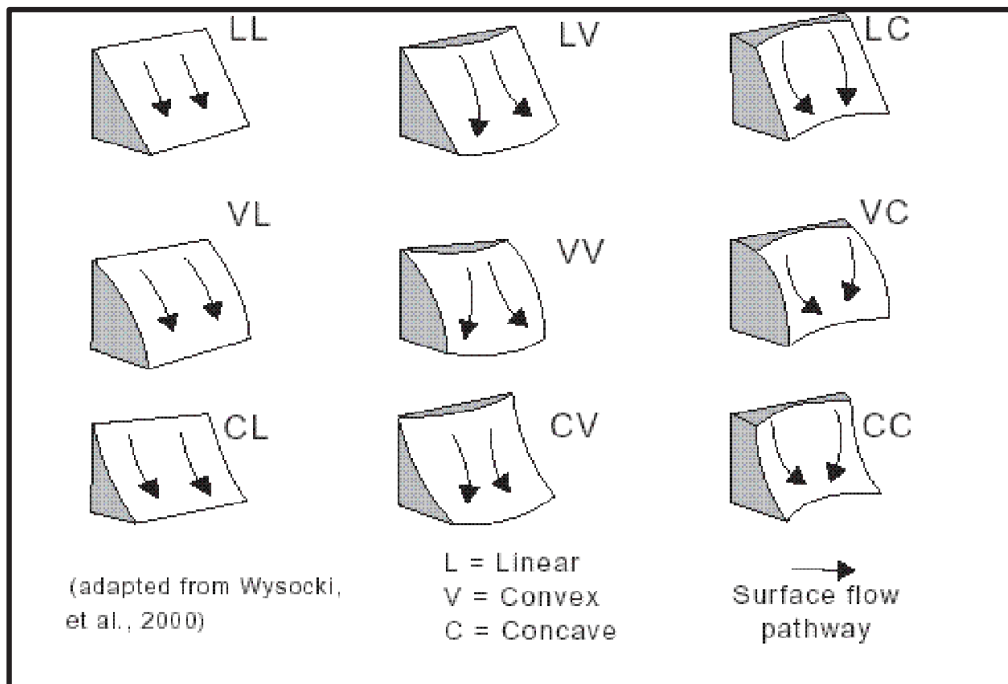
Figure 6.1. Profile and planform terrain forms (Schoenenberger et al., 2002).
