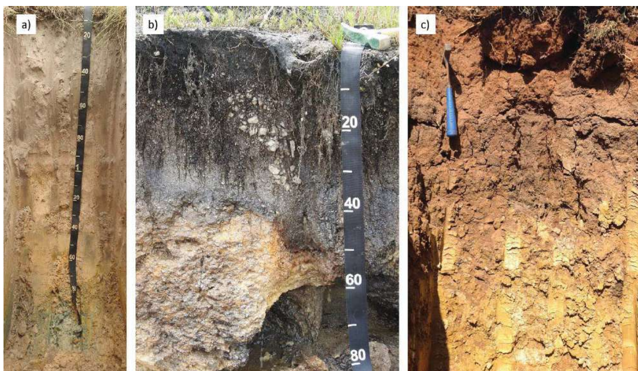
Figure 5.2. Examples of interflow soils: a) Interflow (soil/bedrock) – notice grey colours at the bottom of the profile, b) Interflow (shallow) – water exiting in grey albic between 300 and 500 mm and c) Interflow (slow) – morphological properties of saturation are present but high clay contents limit lateral flow.
