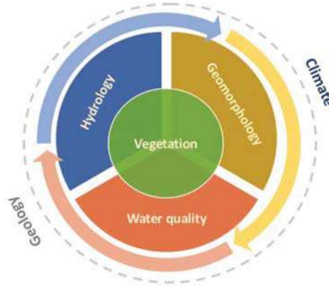
Figure 7.2. Four modules to assess wetland present ecological status using the WET-Health method (MacFarlane et al., 2020)
