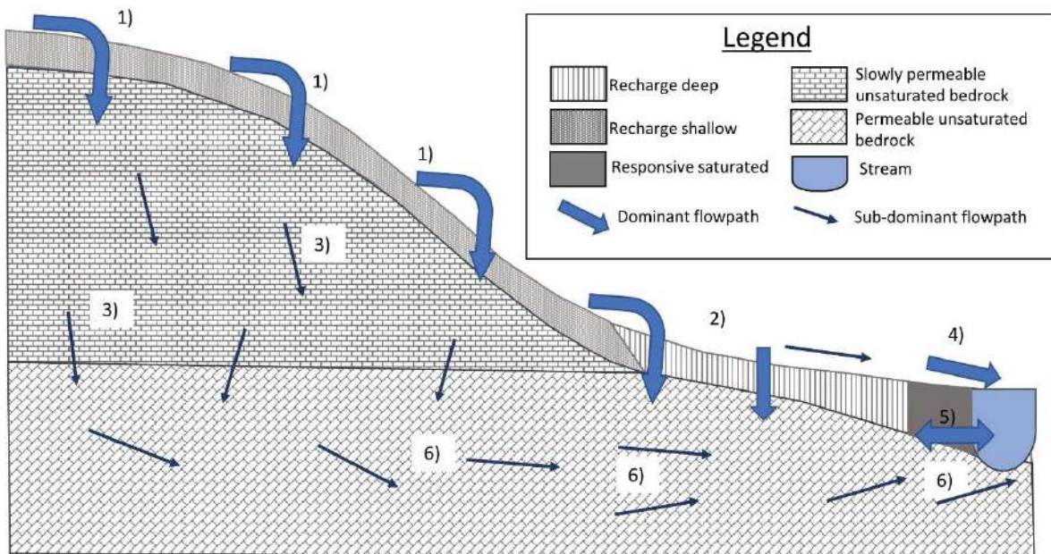
Figure 11.6. Simplified conceptual hydropedological response of the site (arrow number referred to in the text).
