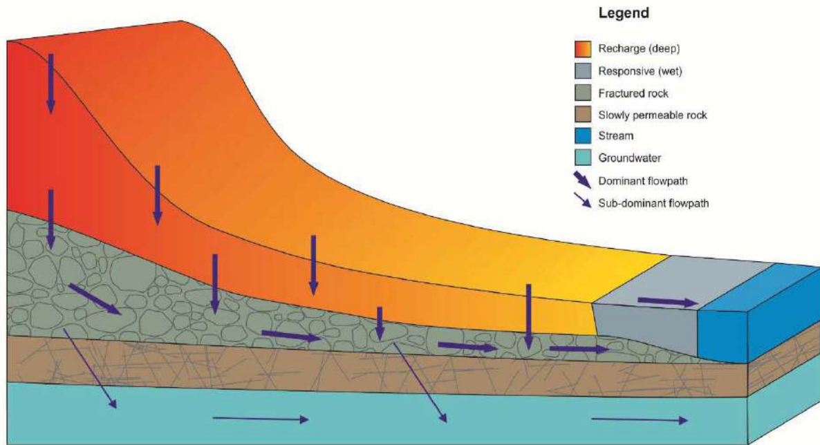
Figure 6.7. Conceptual hydrological response of a Class 6 hillslope.
