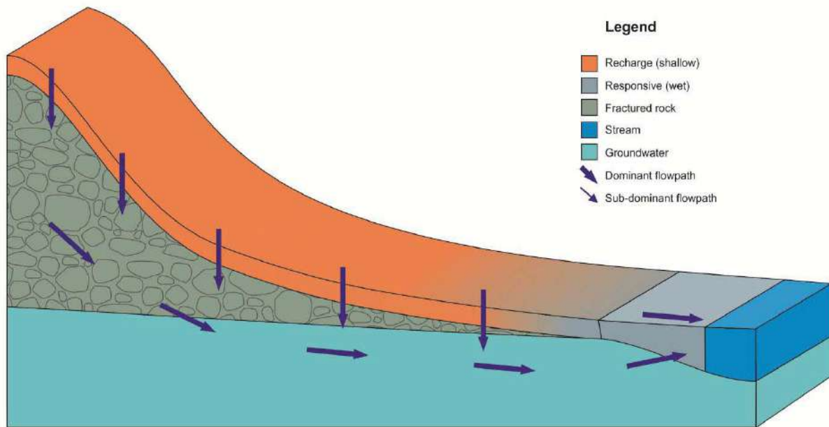
Figure 6.4. Conceptual hydrological response of a Class 3 hillslope.
