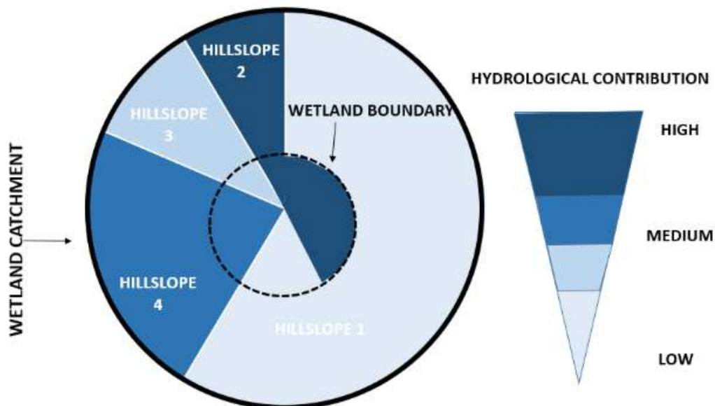
Figure 7.3. A generalised wetland catchment, divided into hillslopes, and depicting both the wetland (within the wetland boundary) and terrestrial components of the hillslopes. Hillslopes are rated according to their hydrological contribution.
