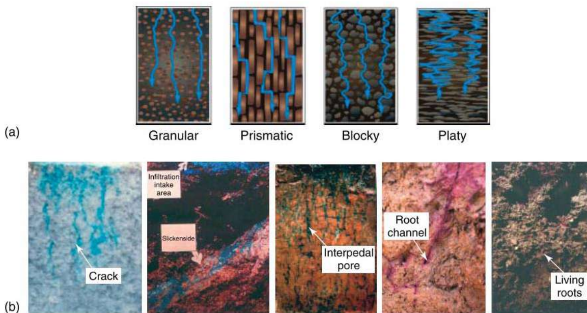
Figure 3.5. a) Conceptual model of flowpaths in differently structured soils, and b) Soil structure influence on preferential flowpaths (Lin et al., 2008).
