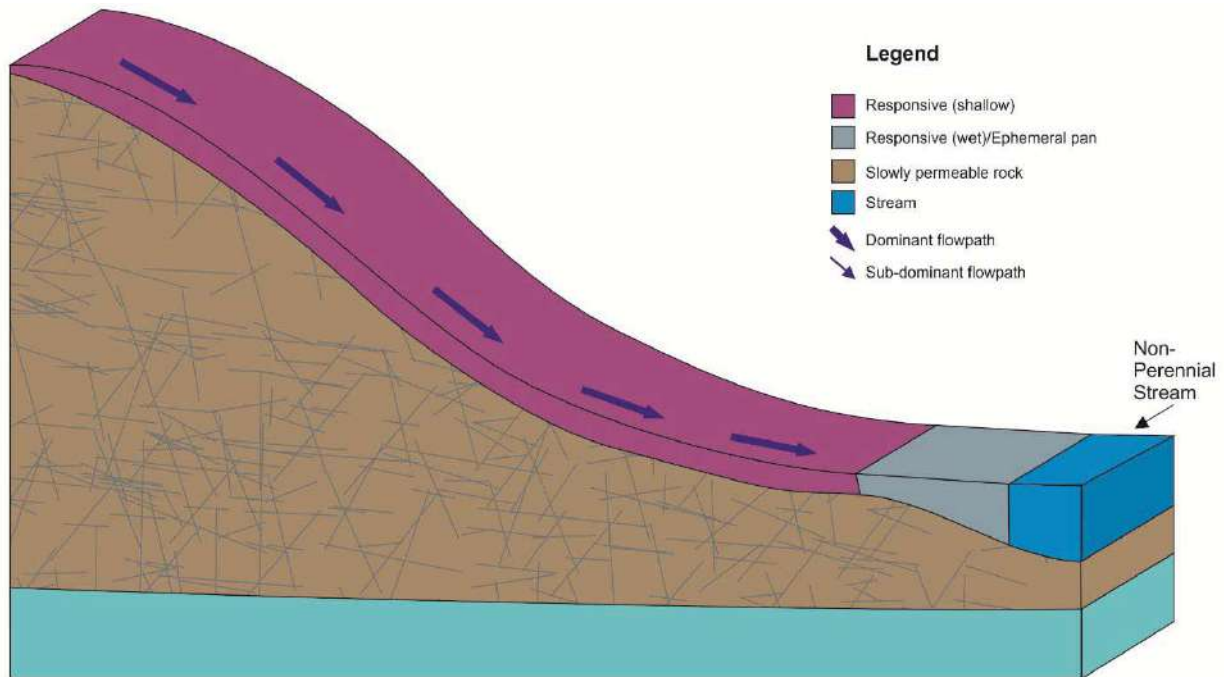
Figure 6.10. Conceptual hydrological response of a Class 9 hillslope.
