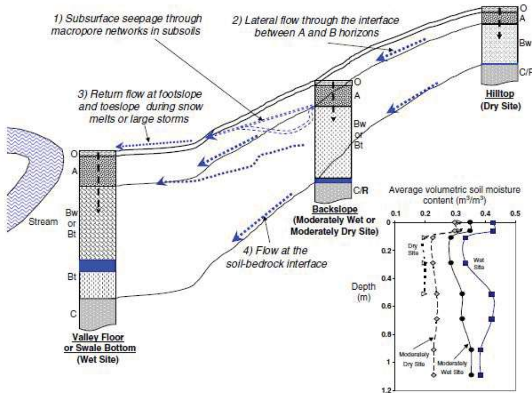
Figure 2.3. Subsurface lateral flowpaths at hillslope scale (Lin et al., 2006).
