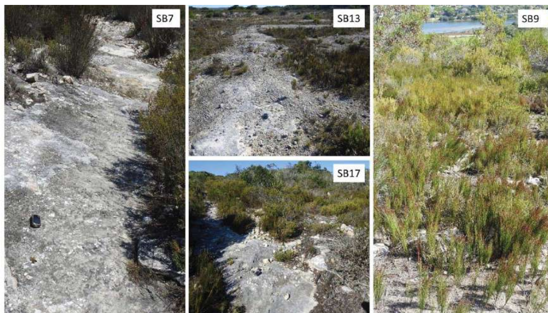
Figure 11.4. Solid carbonate and rock outcrops on the site, often frequented by Elegia species which occur on temporary to seasonally saturated areas.
