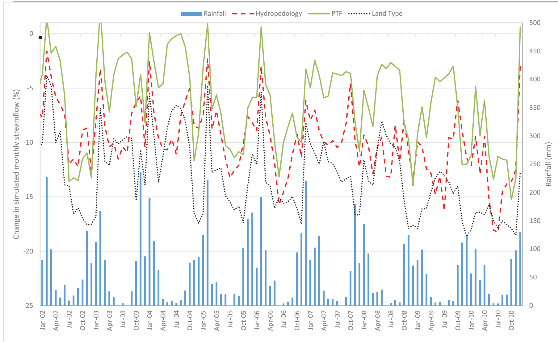
Figure 12.6. Difference (%) between before and after streamflow simulations using various soil inputs for the Mpumalanga Highveld catchment.
