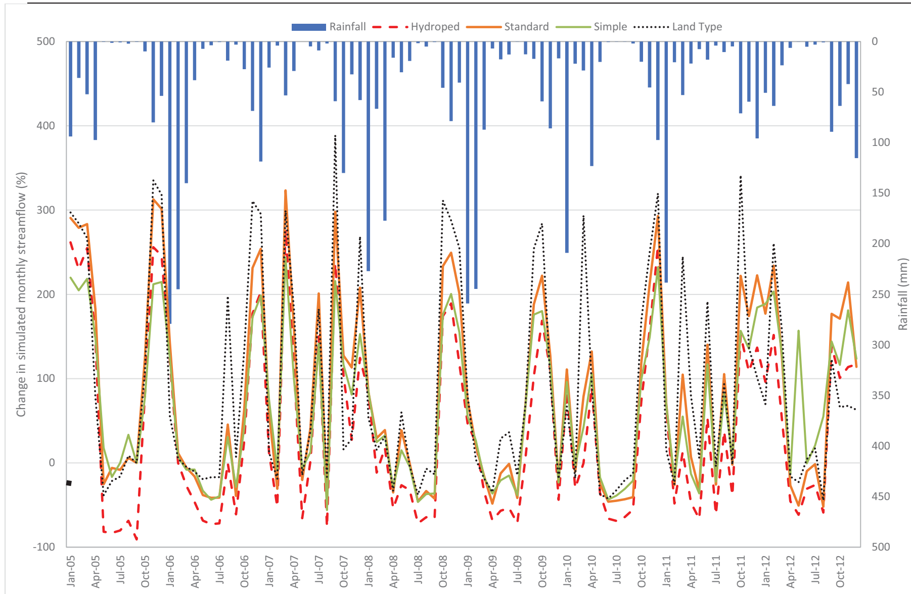
Figure 12.4. Difference (%) between before and after streamflow simulations using various soil inputs for the Cosmo City catchment.
