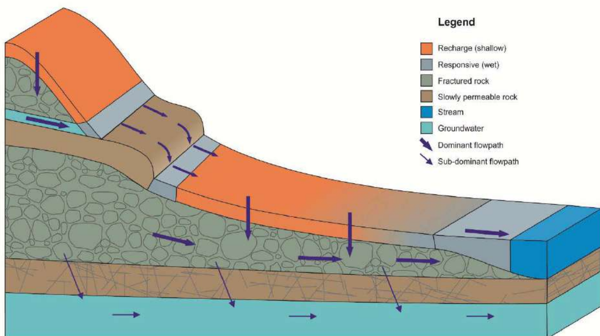
Figure 6.6. Conceptual hydrological response of a Class 5 hillslope.
