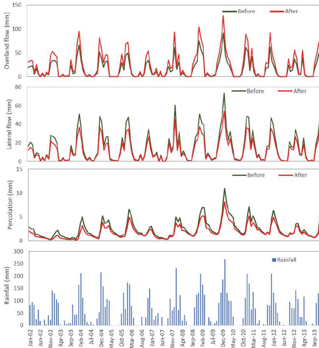
Figure 10.1. Example of a time-step representation of different water balance components obtained from the model.
