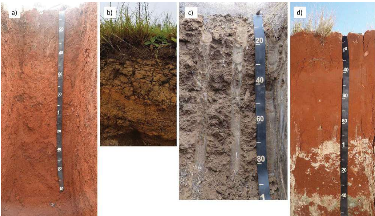
Figure 5.1. Examples of recharge soils: a) Recharge (deep), b) Recharge (shallow), c) Recharge (slow) – high clay contents limit fast vertical drainage and d) Recharge (slow) – lime accumulations indicate insufficient leaching.
