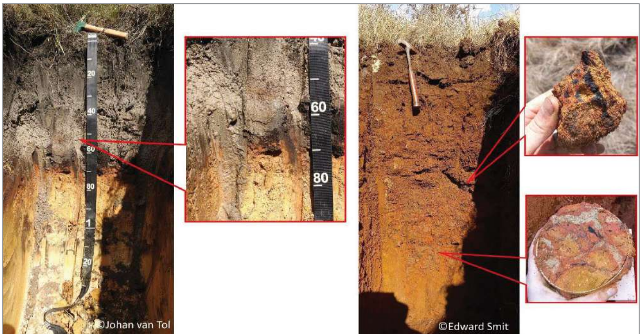
Figure 8.2. Clear photographs with scale and focussing on morphological properties of interest adds value to the report.
