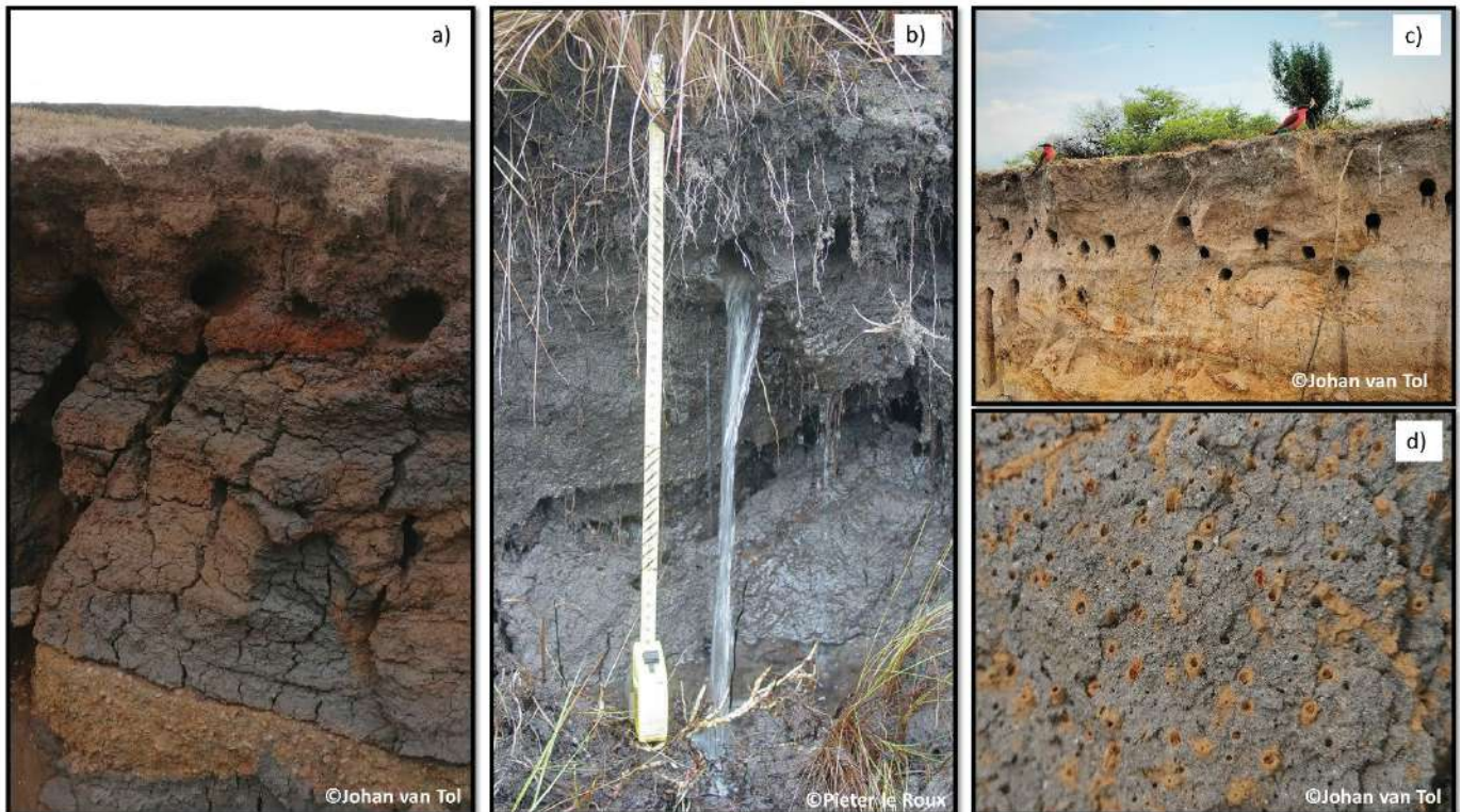
Figure 3.3. Macropores a) ice rat burrows above structural macropores in a degraded peatland in the Lesotho Highlands, b) water flowing out of an animal burrow after heavy rainfall in Weatherley, c) Carmine bee-eater nests serves as macropores in Dundee soils in the Zambezia region, and d) dead root channel macropores in a peat horizon.
